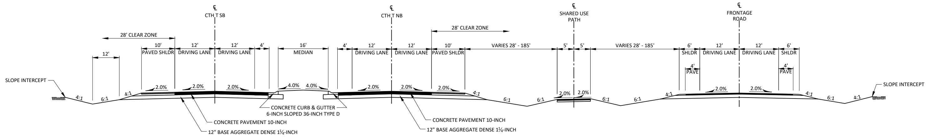
TYPICAL FINISHED SECTION ALTERNATE 3
