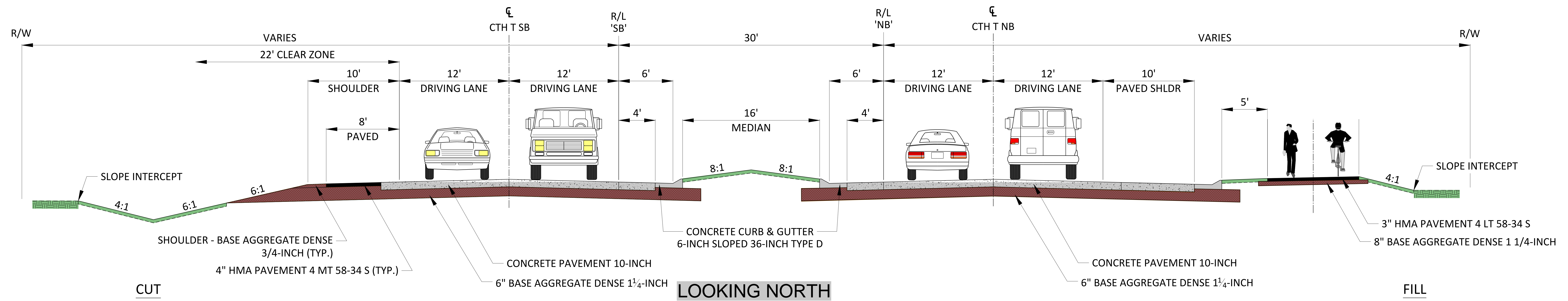
LOOKING NORTH TYPICAL FINISHED SECTION - URBAN CTH T
