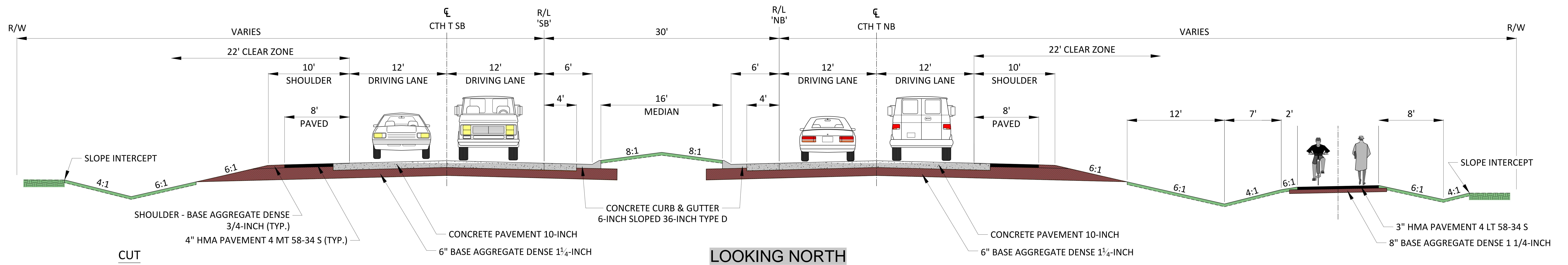
LOOKING NORTH TYPICAL FINISHED SECTION - URBAN CTH T
